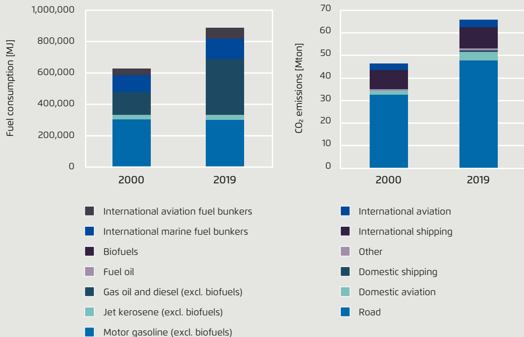
South Africa: Marine fuel bunkers are a major demand segment (left) but overall emissions are dominated by road transport (right)
