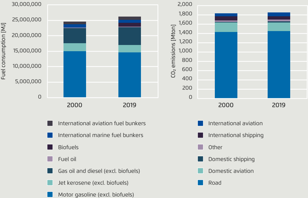
United States: Fuel consumption dominated by petroleum (left) with slight increase in overall emissions (right)
