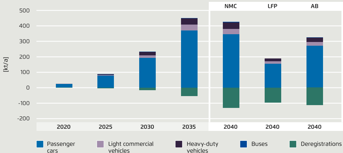
Comparison of primary raw material demand and secondary raw material potential for nickel in the three scenarios considered in the EU-27 in kt/a 2020–2040
