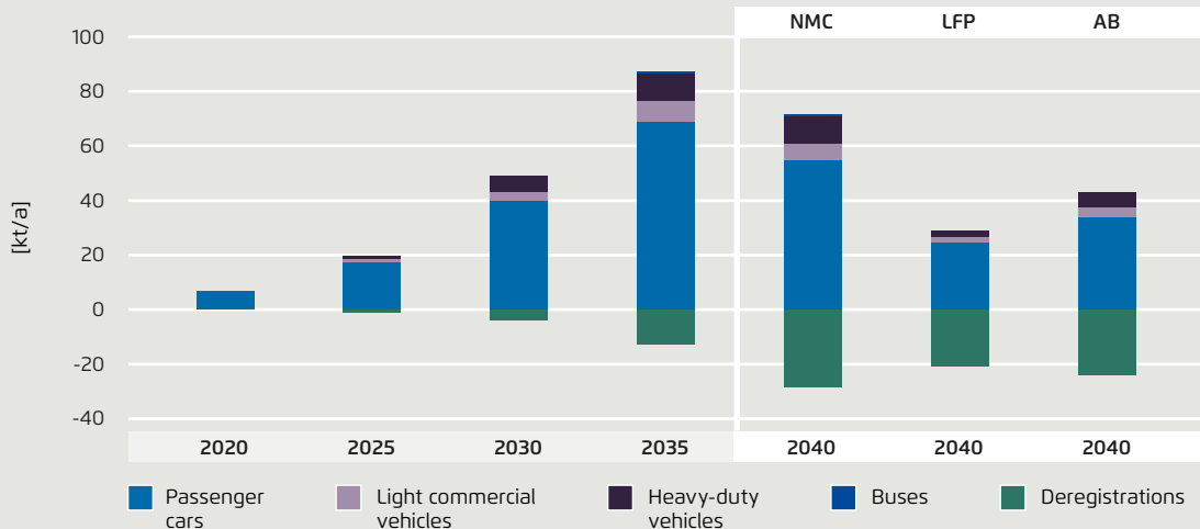
Comparison of primary raw material demand and secondary raw material potential for cobalt in the three scenarios considered in the EU-27 in kt/a 2020–2040
